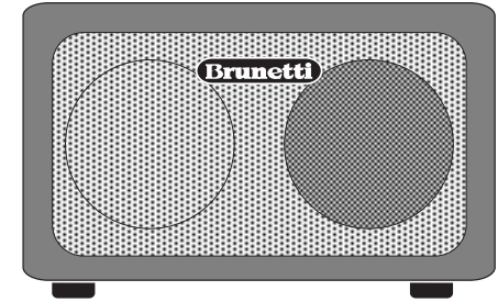
CABINET 2x12" USING ONLY 1 SPEAKER 16Ω - 16Ω
